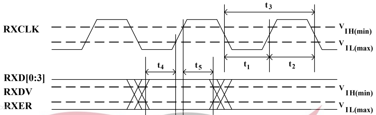
Figure 8. MII Reception Cycle Timing-1
