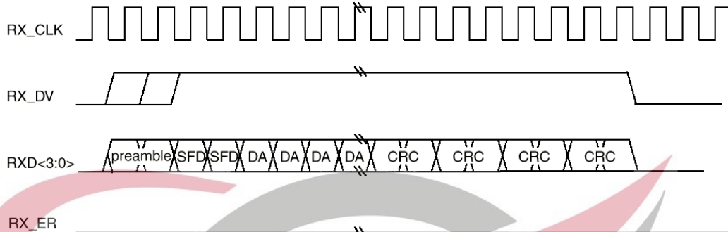
Figure 16. MDC/MDIO PHY to MAC Reception Without Error
