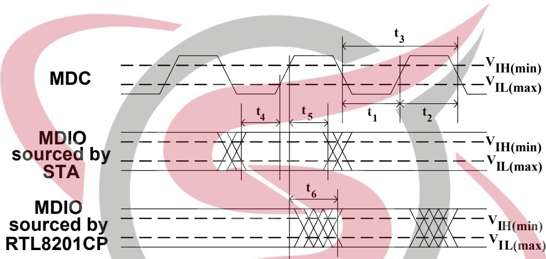
Figure 14. MDC/MDIO Timing
